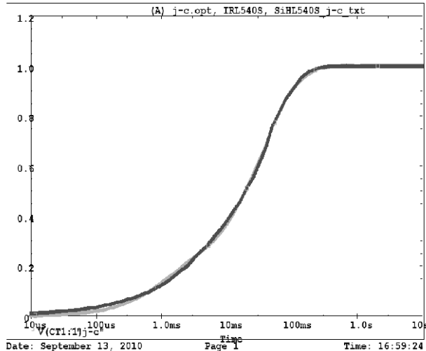
IRL540S, SiHL540S Tank j-c Temperature: 27.0
