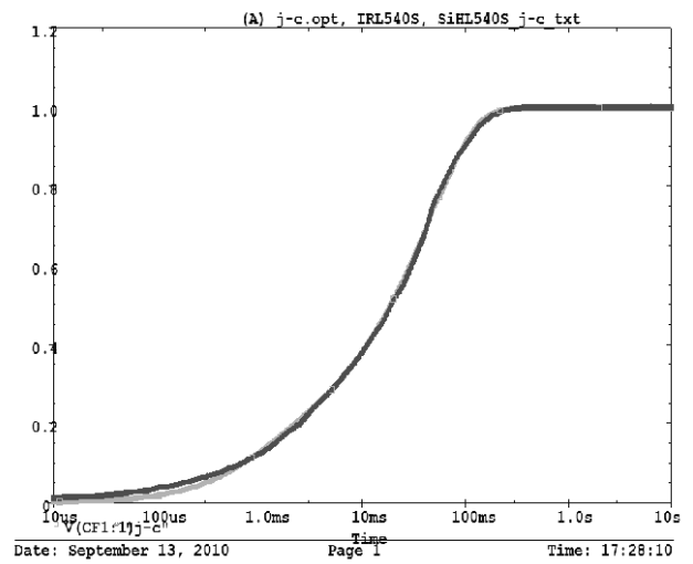
IRL540S, SiHL540S Filter j-c Temperature: 27.0
